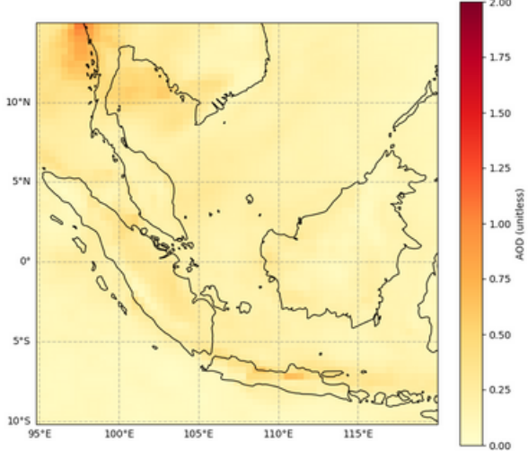
Total Aerosol Optical Depth, AOD at 550 nm, 2024-01-29T00
