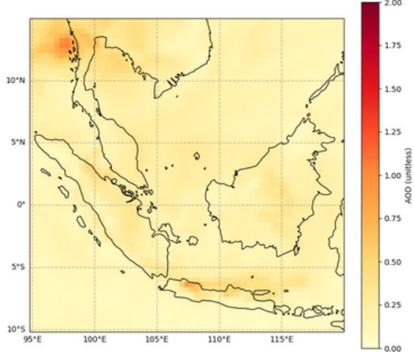
Total Aerosol Optical Depth, AOD at 550 nm, 2024-01-30T00
