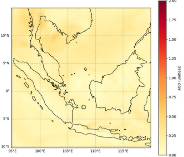
Total Aerosol Optical Depth, AOD at 550 nm, 2024-01-19T00
