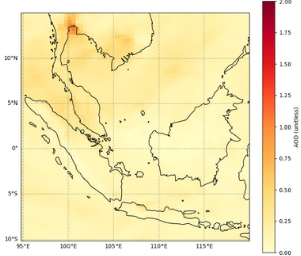
Total Aerosol Optical Depth, AOD at 550 nm, 2024-01-20T00
