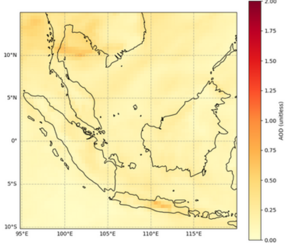
Total Aerosol Optical Depth, AOD at 550 nm, 2024-01-27T00
