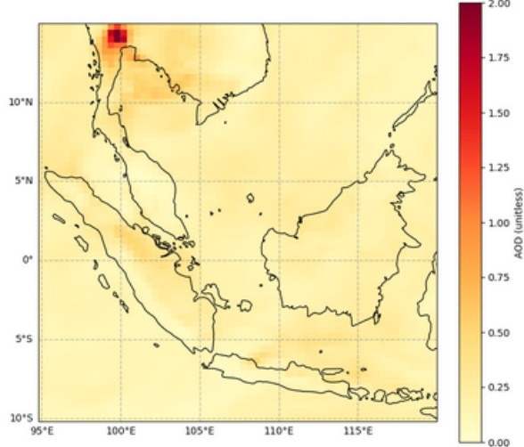
Total Aerosol Optical Depth, AOD at 550 nm, 2024-01-23T00
