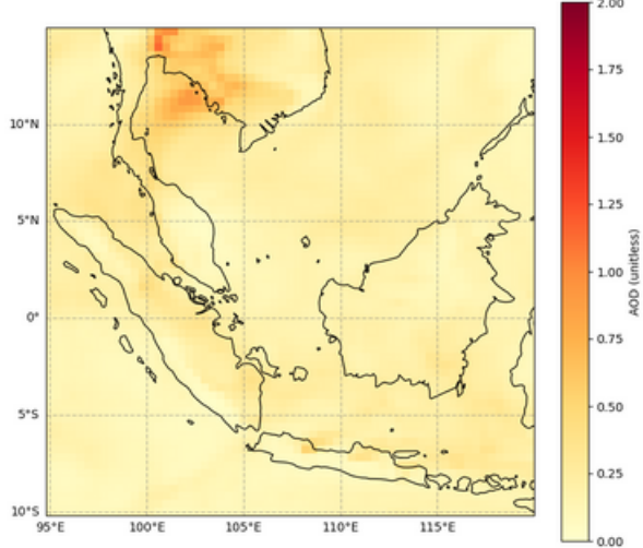
Total Aerosol Optical Depth, AOD at 550 nm, 2024-01-22T00
