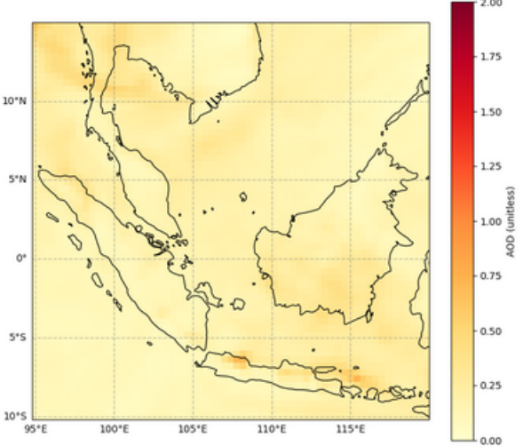
Total Aerosol Optical Depth, AOD at 550 nm, 2024-01-25T00
