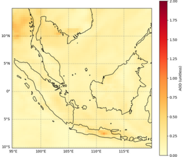
Total Aerosol Optical Depth, AOD at 550 nm, 2024-01-28T00
