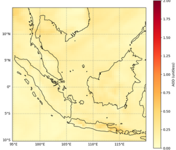
Total Aerosol Optical Depth, AOD at 550 nm, 2024-01-26T00
