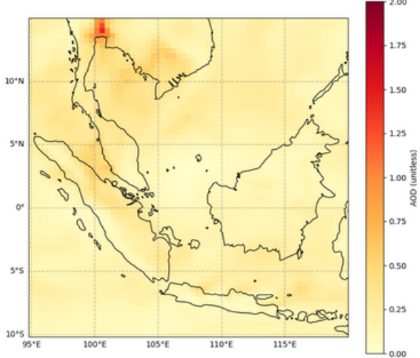
Total Aerosol Optical Depth, AOD at 550 nm, 2024-01-21T00
