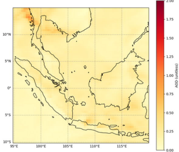
Total Aerosol Optical Depth, AOD at 550 nm, 2024-01-24T00
