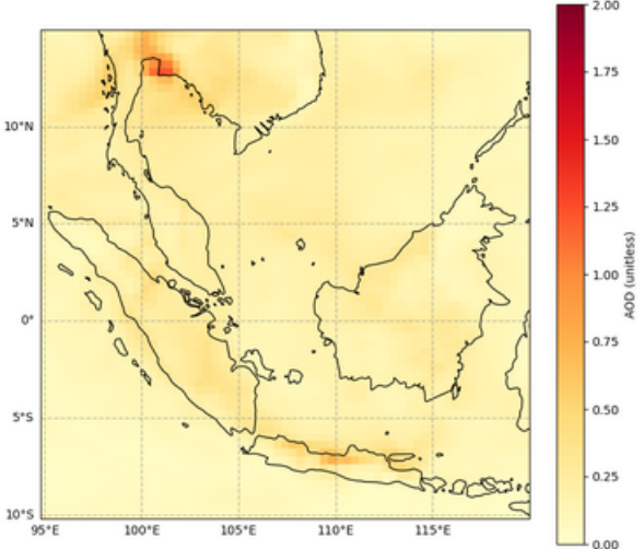
Total Aerosol Optical Depth, AOD at 550 nm, 2024-01-31T00
