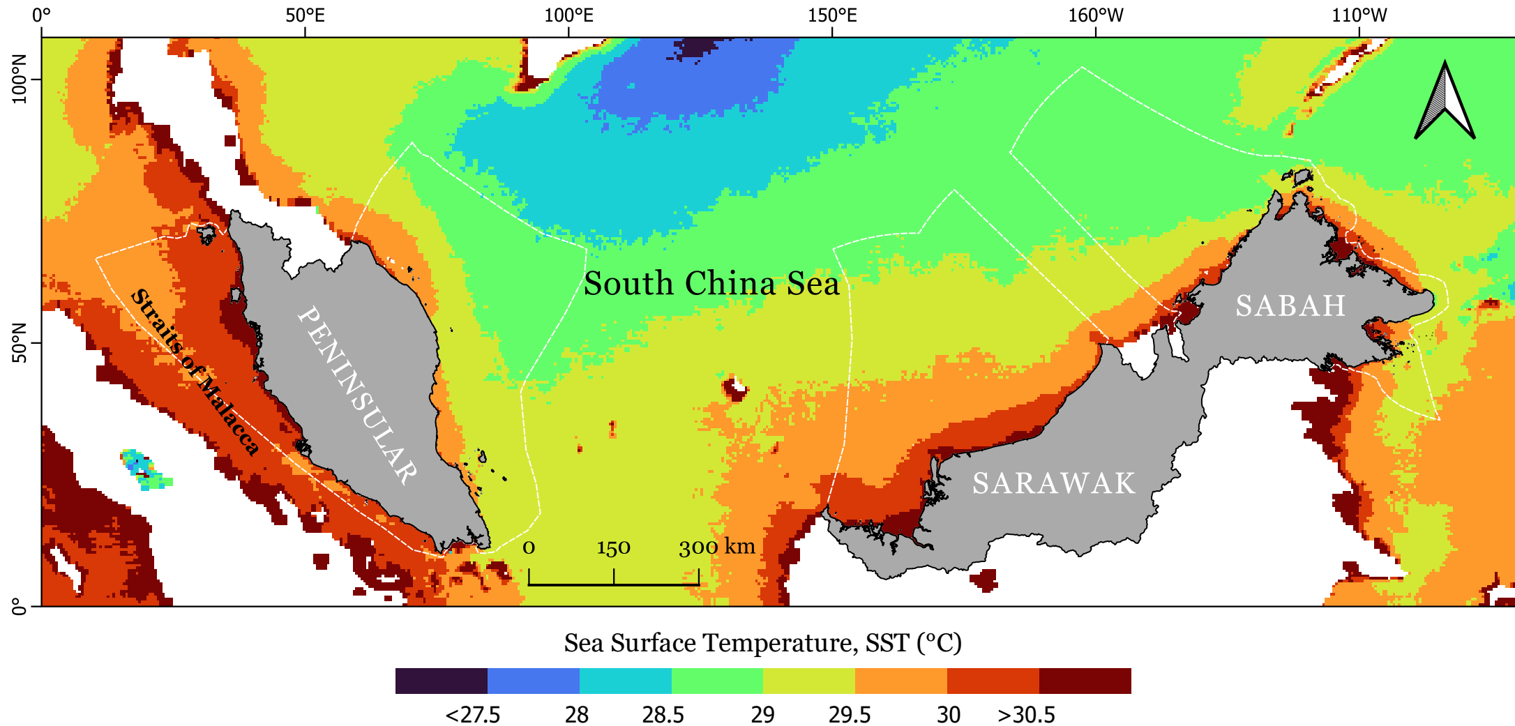
Five Years Time Averaged Map of Sea Surface Temperature in Malaysia, °C (2003-2007)
