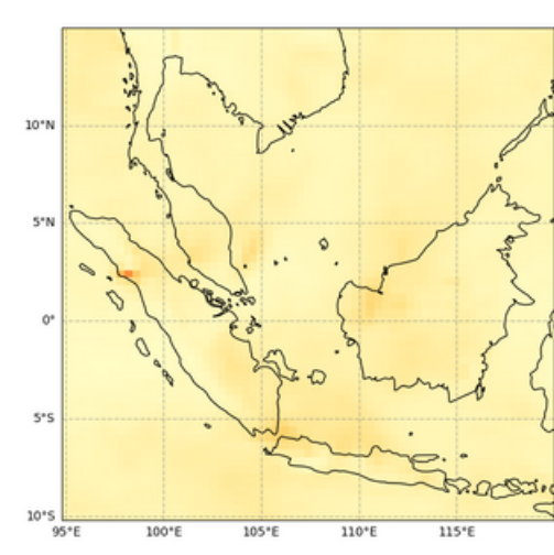
Total Aerosol Optical Depth at 550 nm, 2022-08-17T00
