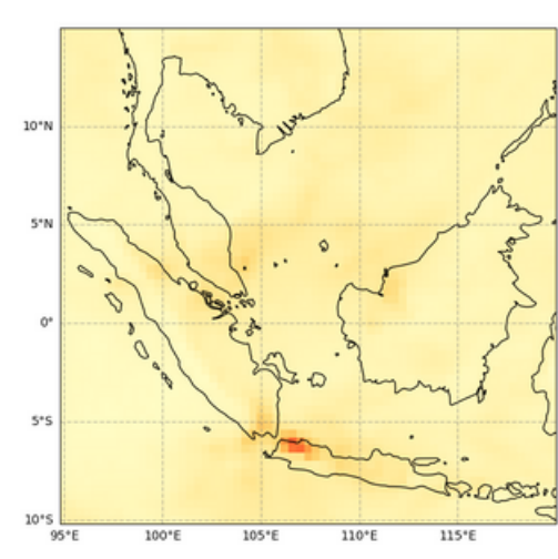
Total Aerosol Optical Depth at 550 nm, 2022-08-16T00
