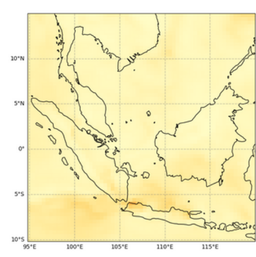
Total Aerosol Optical Depth at 550 nm, 2022-08-05T00
