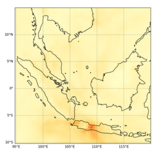
Total Aerosol Optical Depth at 550 nm, 2022-08-02T00
