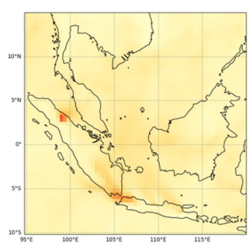
Total Aerosol Optical Depth at 550 nm, 2022-08-08T00
