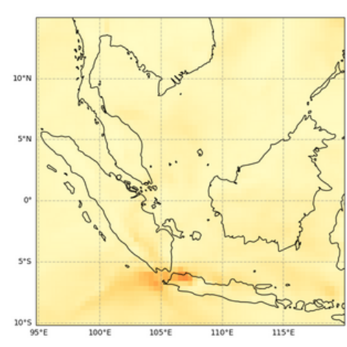
Total Aerosol Optical Depth at 550 nm, 2022-08-04T00
