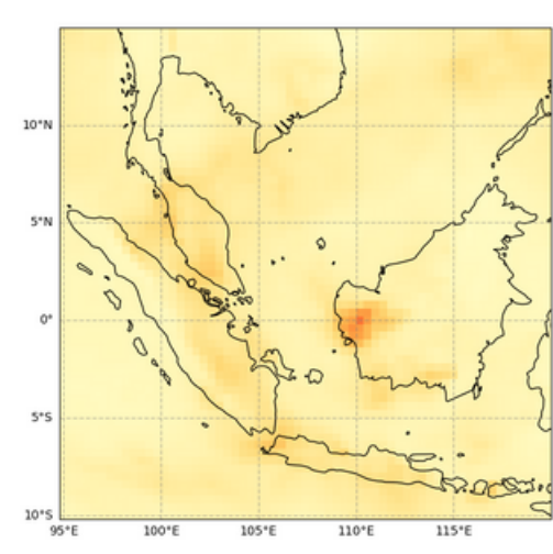
Total Aerosol Optical Depth at 550 nm, 2022-08-13T00
