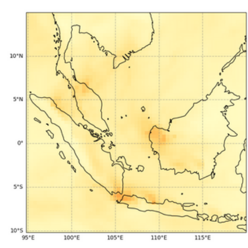
Total Aerosol Optical Depth at 550 nm, 2022-08-12T00
