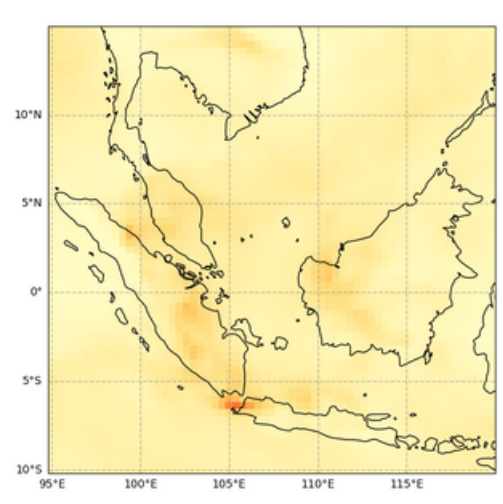
Total Aerosol Optical Depth at 550 nm, 2022-08-10T00
