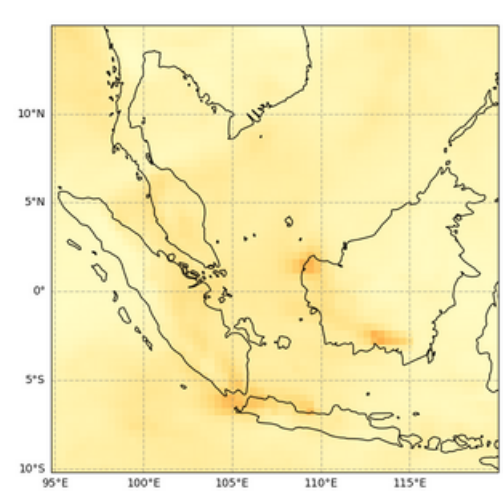
Total Aerosol Optical Depth at 550 nm, 2022-08-11T00
