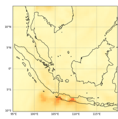
Total Aerosol Optical Depth at 550 nm, 2022-08-01T00
