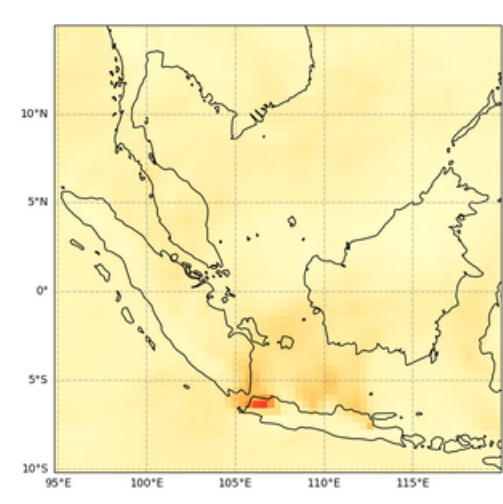
Total Aerosol Optical Depth at 550 nm, 2022-08-07T00
