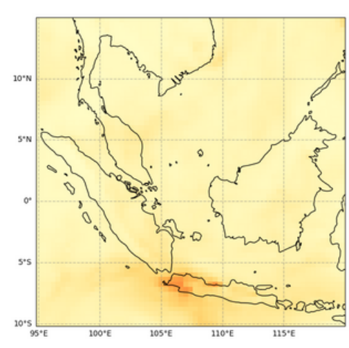
Total Aerosol Optical Depth at 550 nm, 2022-08-03T00
