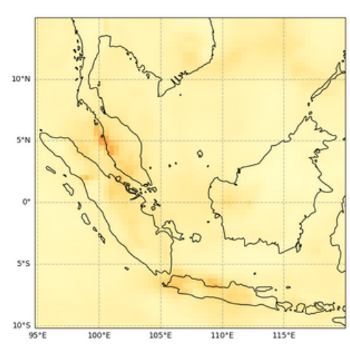
Total Aerosol Optical Depth at 550 nm, 2022-08-14T00
