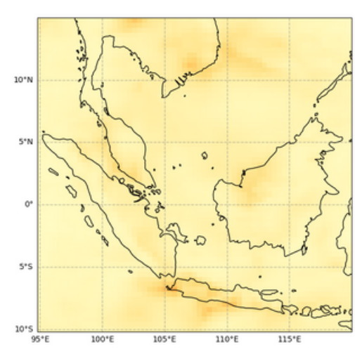
Total Aerosol Optical Depth at 550 nm, 2022-08-15T00
