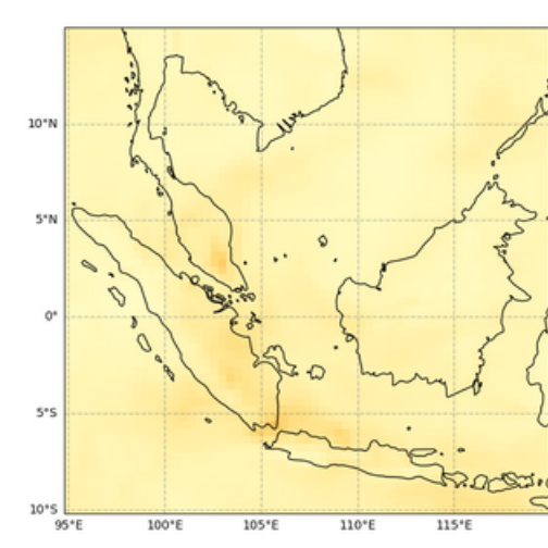
Total Aerosol Optical Depth at 550 nm, 2022-08-18T00
