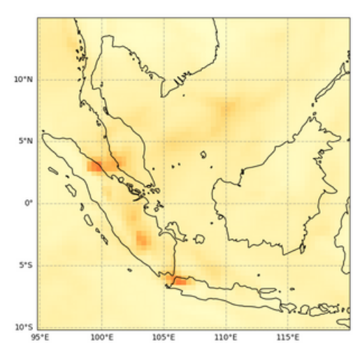
Total Aerosol Optical Depth at 550 nm, 2022-08-09T00
