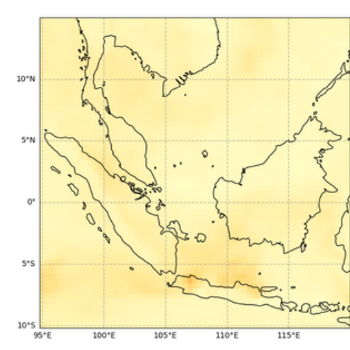
Total Aerosol Optical Depth at 550 nm, 2022-08-06T00
