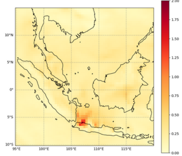
Total Aerosol Optical Depth at 550 nm, 2023-07-26T00
