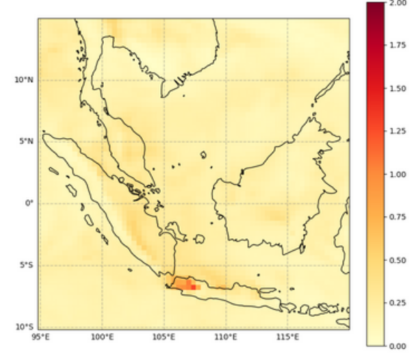
Total Aerosol Optical Depth at 550 nm, 2023-07-23T00
