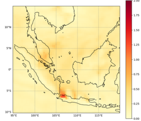
Total Aerosol Optical Depth at 550 nm, 2023-07-27T00
