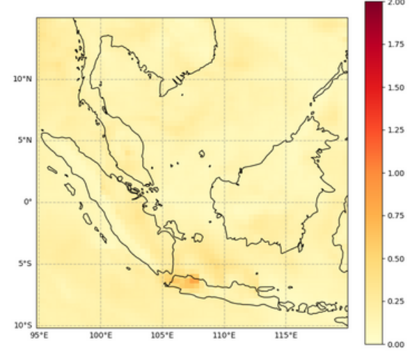
Total Aerosol Optical Depth at 550 nm, 2023-07-21T00
