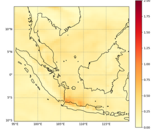
Total Aerosol Optical Depth at 550 nm, 2023-07-25T00
