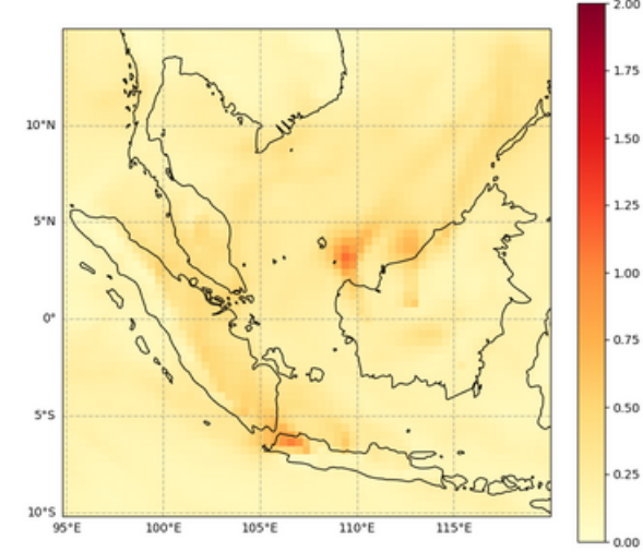
Total Aerosol Optical Depth at 550 nm, 2023-07-30T00
