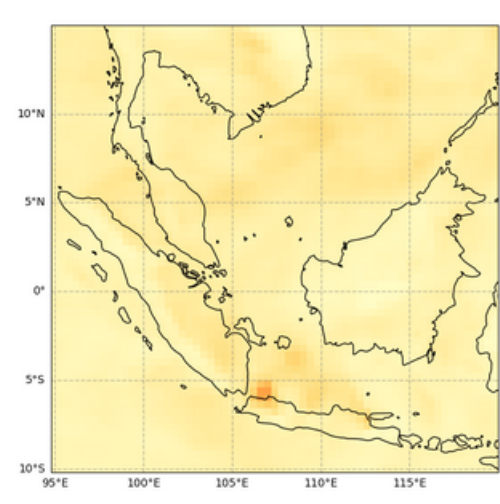
Total Aerosol Optical Depth at 550 nm, 2023-07-16T00
