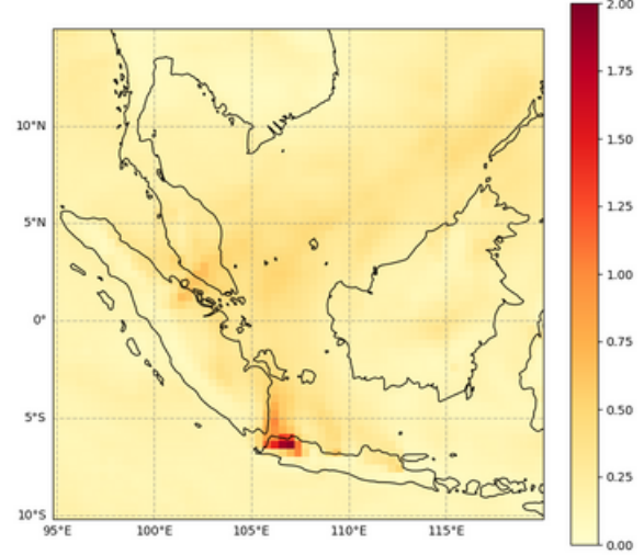
Total Aerosol Optical Depth at 550 nm, 2023-07-28T00
