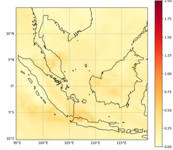
Total Aerosol Optical Depth at 550 nm, 2023-07-19T00
