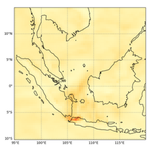
Total Aerosol Optical Depth at 550 nm, 2023-07-15T00
