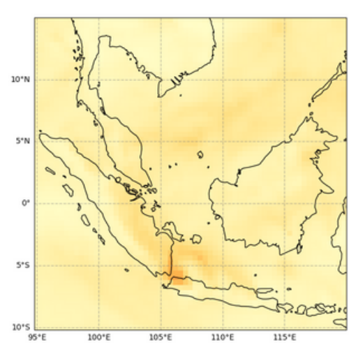
Total Aerosol Optical Depth at 550 nm, 2023-07-17T00
