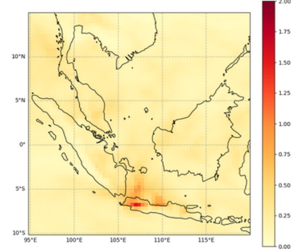
Total Aerosol Optical Depth at 550 nm, 2023-07-24T00
