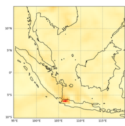
Total Aerosol Optical Depth at 550 nm, 2023-07-13T00
