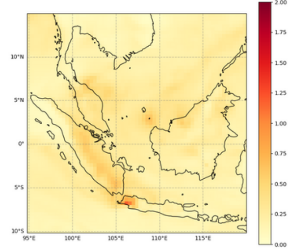
Total Aerosol Optical Depth at 550 nm, 2023-07-31T00
