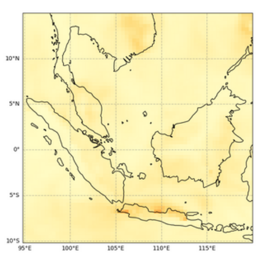
Total Aerosol Optical Depth at 550 nm, 2023-07-11T00
