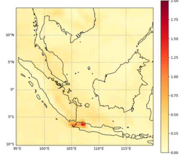
Total Aerosol Optical Depth at 550 nm, 2023-07-22T00
