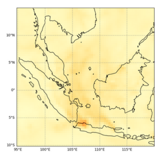
Total Aerosol Optical Depth at 550 nm, 2023-07-01T00
