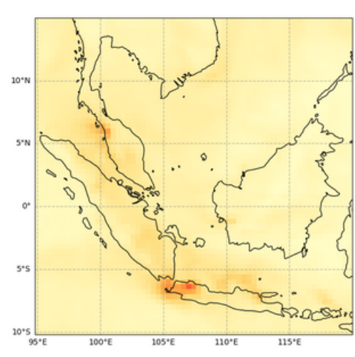
Total Aerosol Optical Depth at 550 nm, 2023-07-04T00
