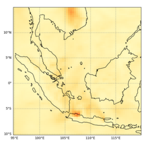
Total Aerosol Optical Depth at 550 nm, 2023-07-14T00
