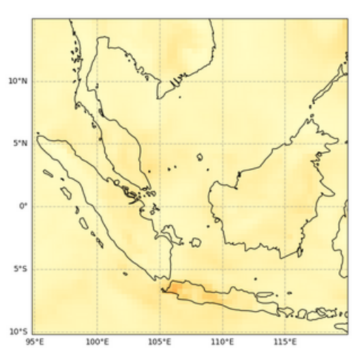
Total Aerosol Optical Depth at 550 nm, 2023-07-10T00
