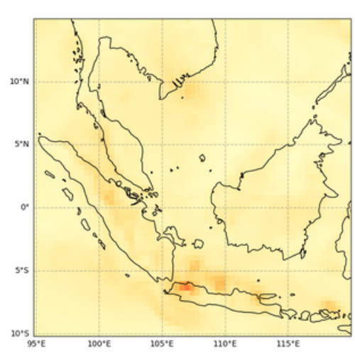
Total Aerosol Optical Depth at 550 nm, 2023-07-05T00
