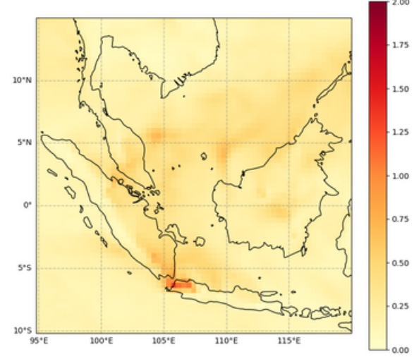
Total Aerosol Optical Depth at 550 nm, 2023-07-29T00
