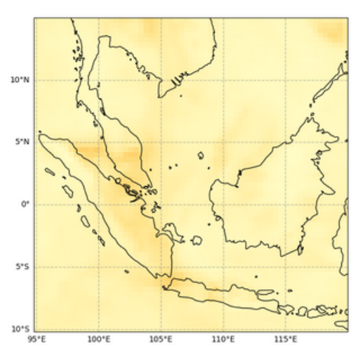
Total Aerosol Optical Depth at 550 nm, 2023-07-09T00
