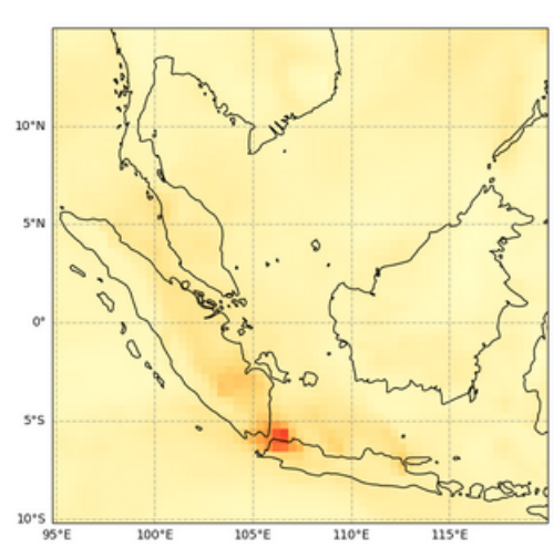
Total Aerosol Optical Depth at 550 nm, 2023-07-03T00
