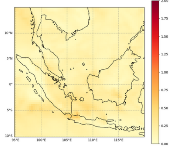
Total Aerosol Optical Depth at 550 nm, 2023-07-20T00
