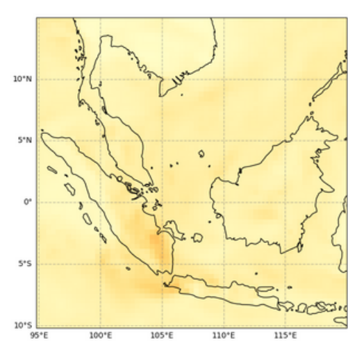
Total Aerosol Optical Depth at 550 nm, 2023-07-18T00
