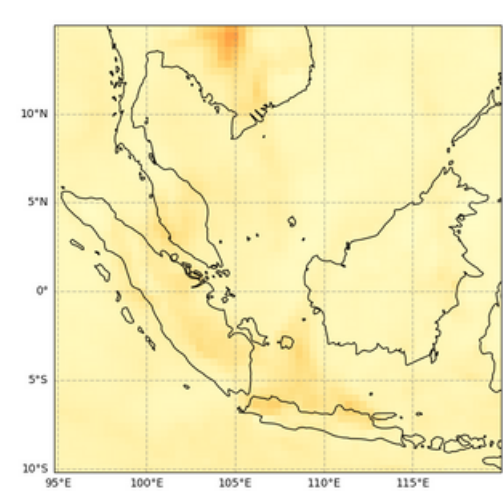
Total Aerosol Optical Depth at 550 nm, 2023-07-07T00
