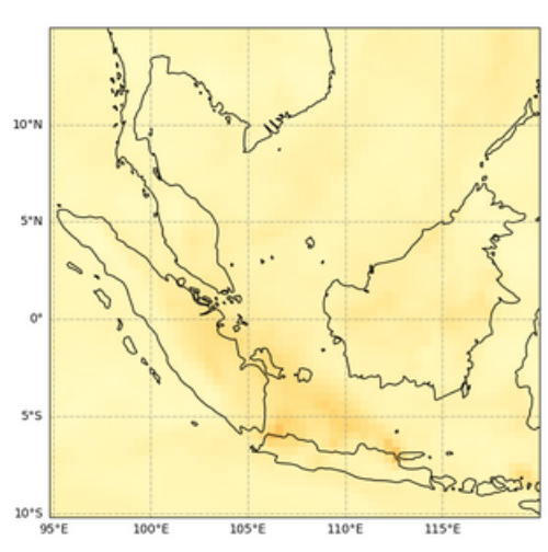
Total Aerosol Optical Depth at 550 nm, 2023-07-02T00
