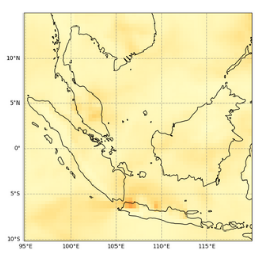
Total Aerosol Optical Depth at 550 nm, 2023-07-12T00
