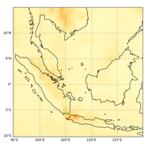
Total Aerosol Optical Depth at 550 nm, 2023-07-08T00
