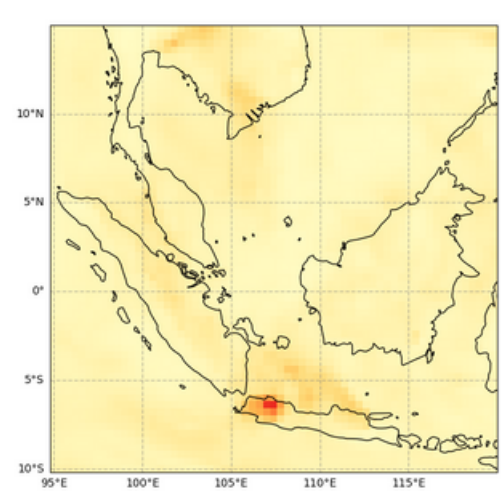
Total Aerosol Optical Depth at 550 nm, 2023-07-06T00
