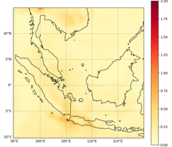
Total Aerosol Optical Depth at 550 nm, 2022-07-28T00
