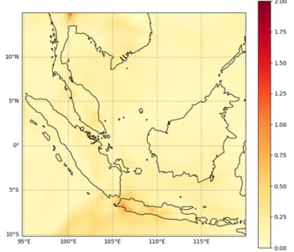
Total Aerosol Optical Depth at 550 nm, 2022-07-29T00
