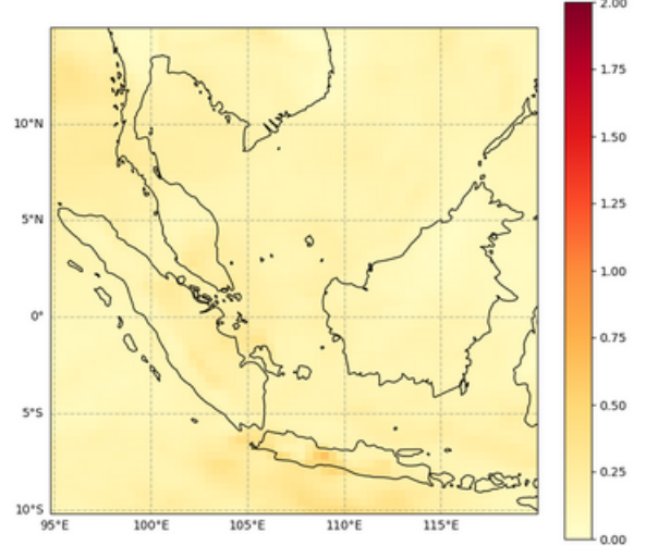
Total Aerosol Optical Depth at 550 nm, 2022-07-14T00
