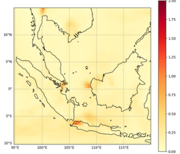
Total Aerosol Optical Depth at 550 nm, 2022-07-24T00
