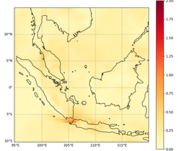
Total Aerosol Optical Depth at 550 nm, 2022-07-18T00
