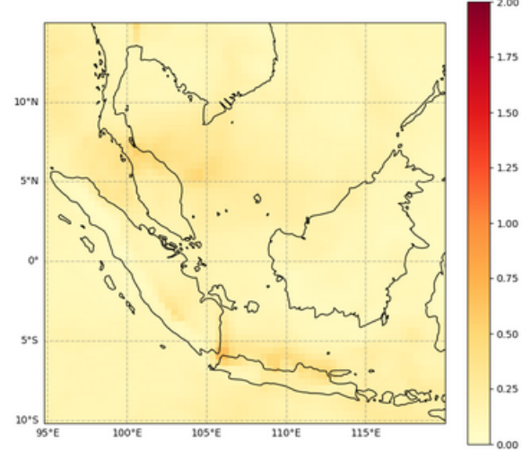
Total Aerosol Optical Depth at 550 nm, 2022-07-17T00
