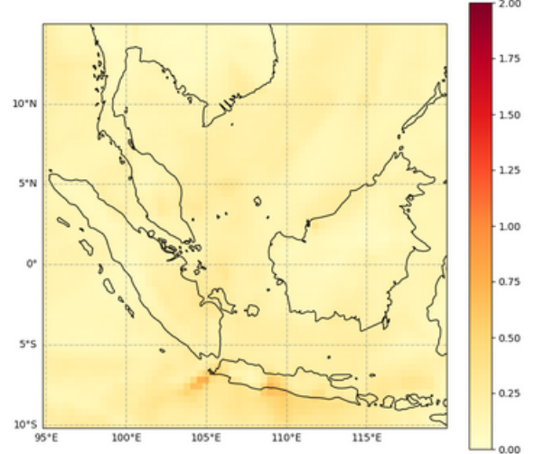
Total Aerosol Optical Depth at 550 nm, 2022-07-05T00
