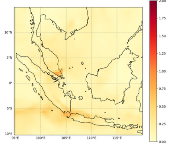
Total Aerosol Optical Depth at 550 nm, 2022-07-22T00
