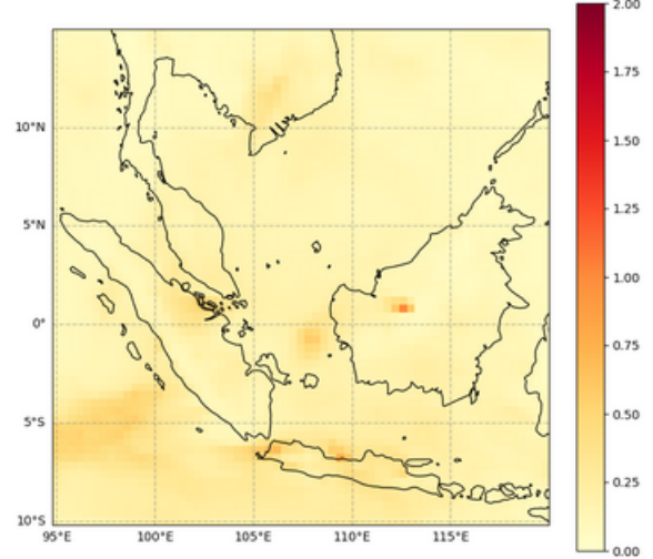
Total Aerosol Optical Depth at 550 nm, 2022-07-23T00
