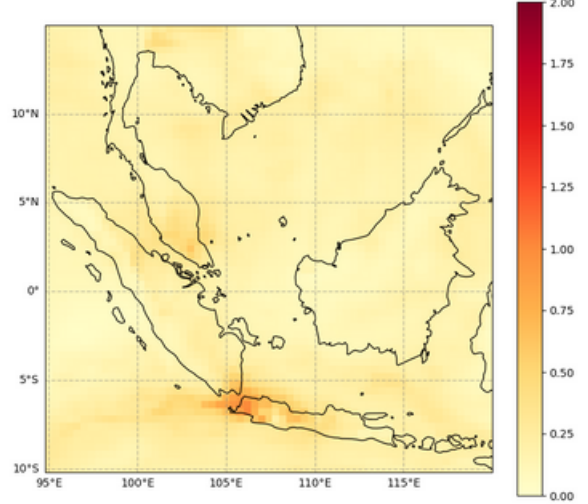
Total Aerosol Optical Depth at 550 nm, 2022-07-20T00
