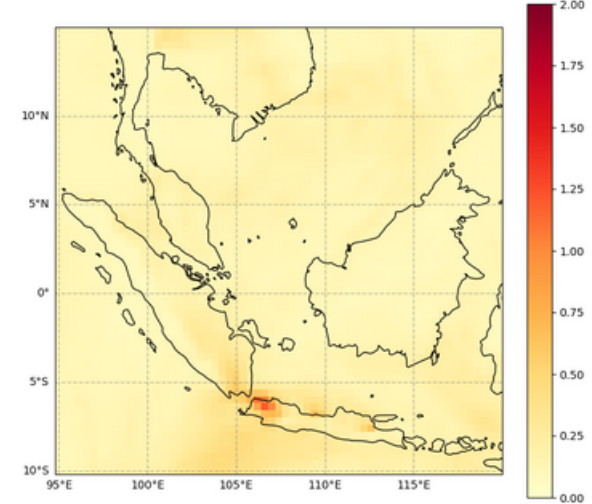
Total Aerosol Optical Depth at 550 nm, 2022-07-31T00
