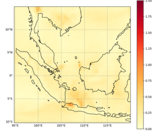
Total Aerosol Optical Depth at 550 nm, 2022-07-25T00
