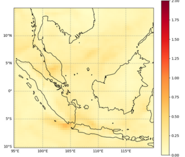
Total Aerosol Optical Depth at 550 nm, 2022-07-11T00
