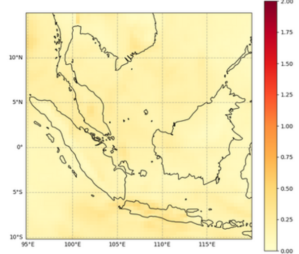
Total Aerosol Optical Depth at 550 nm, 2022-07-16T00
