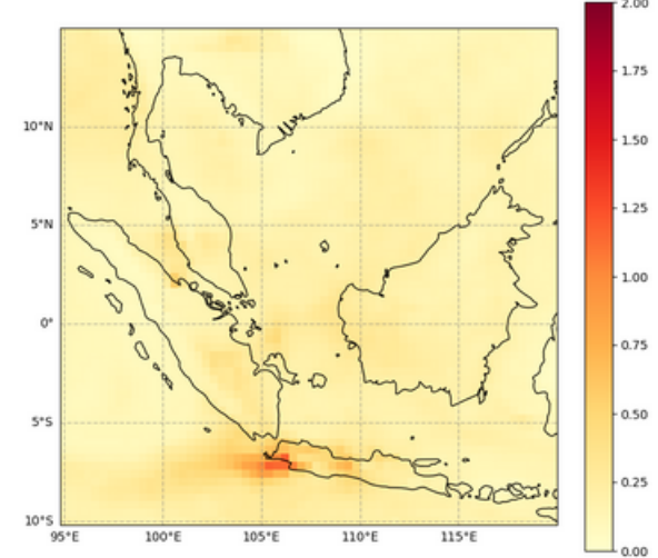
Total Aerosol Optical Depth at 550 nm, 2022-07-13T00
