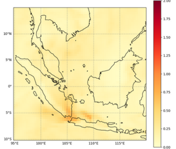
Total Aerosol Optical Depth at 550 nm, 2022-07-02T00
