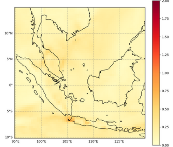
Total Aerosol Optical Depth at 550 nm, 2022-07-04T00
