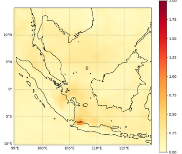
Total Aerosol Optical Depth at 550 nm, 2022-07-09T00
