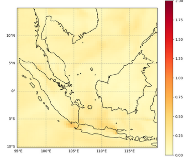
Total Aerosol Optical Depth at 550 nm, 2022-07-01T00
