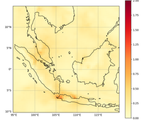
Total Aerosol Optical Depth at 550 nm, 2022-07-19T00
