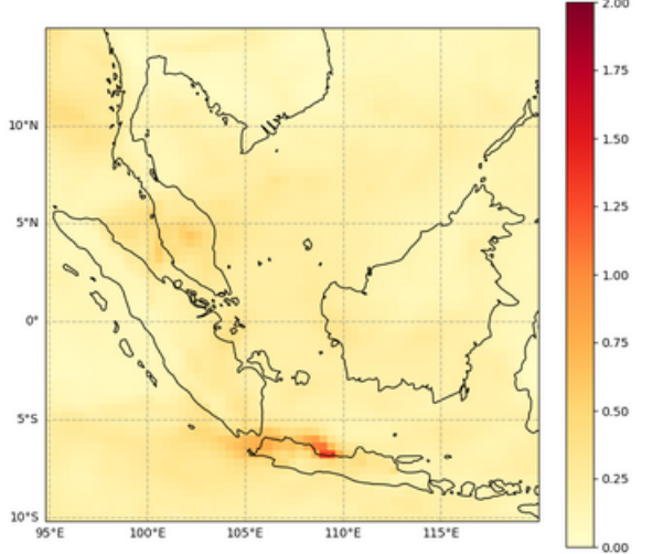
Total Aerosol Optical Depth at 550 nm, 2022-07-12T00
