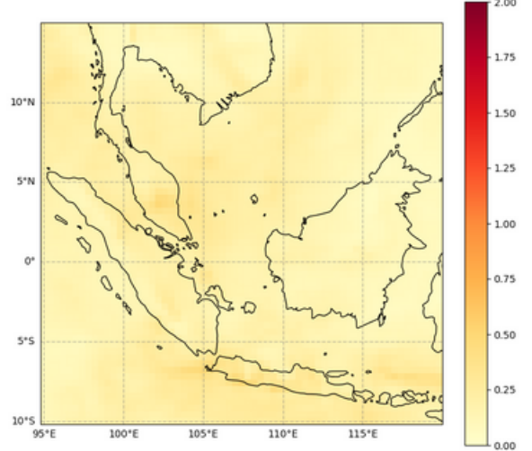
Total Aerosol Optical Depth at 550 nm, 2022-07-15T00
