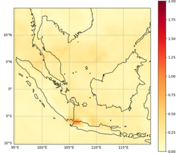
Total Aerosol Optical Depth at 550 nm, 2022-07-10T00
