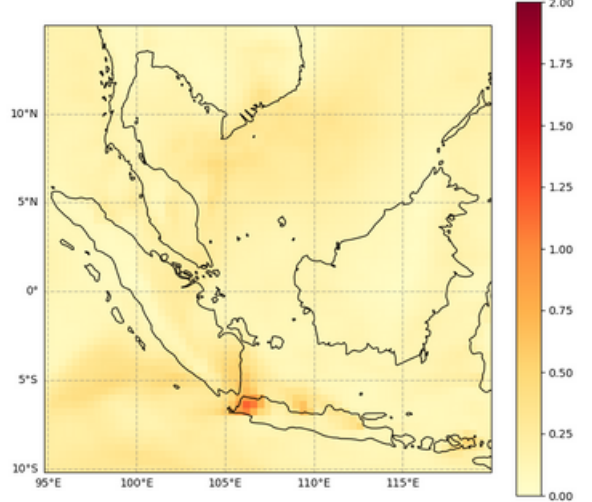
Total Aerosol Optical Depth at 550 nm, 2022-07-03T00
