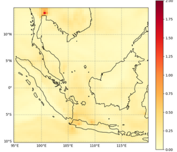
Total Aerosol Optical Depth at 550 nm, 2022-07-26T00
