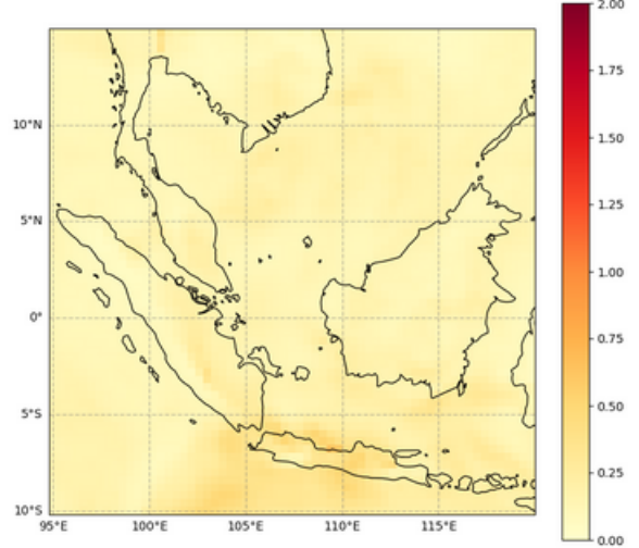
Total Aerosol Optical Depth at 550 nm, 2022-07-30T00
