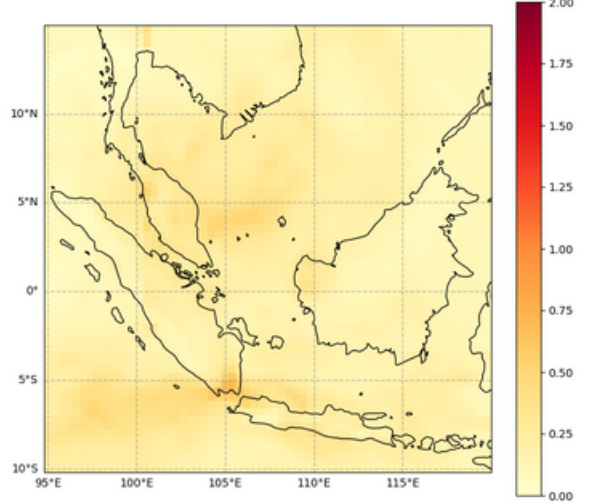
Total Aerosol Optical Depth at 550 nm, 2022-07-21T00
