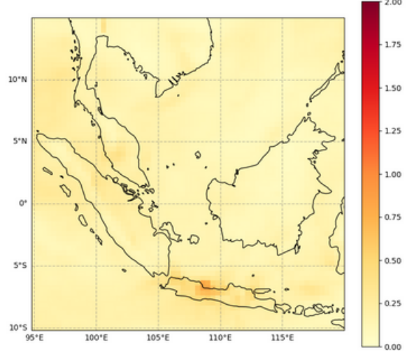
Total Aerosol Optical Depth at 550 nm, 2022-07-06T00
