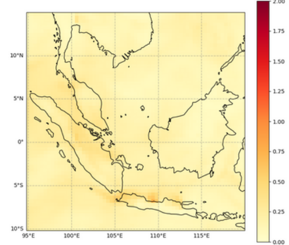
Total Aerosol Optical Depth at 550 nm, 2022-07-07T00
