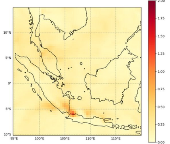
Total Aerosol Optical Depth at 550 nm, 2022-07-08T00
