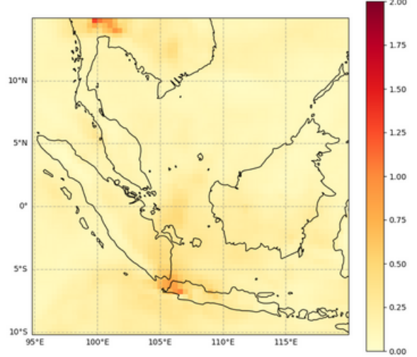
Total Aerosol Optical Depth at 550 nm, 2022-07-27T00
