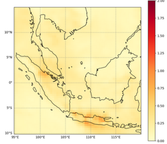
Total Aerosol Optical Depth at 550 nm, 2023-06-20T00
