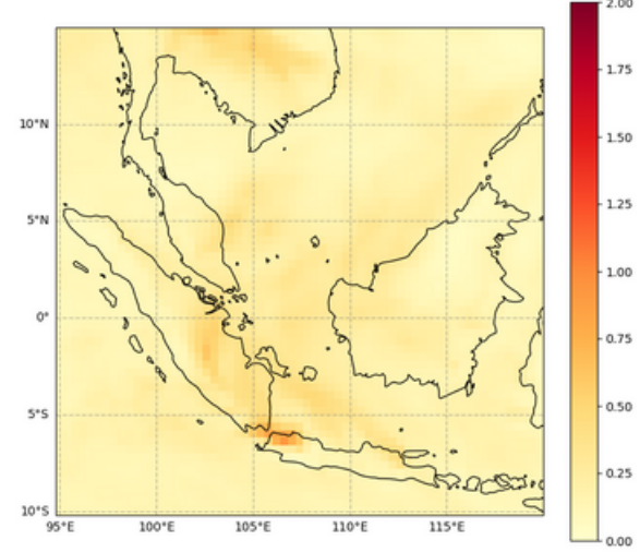
Total Aerosol Optical Depth at 550 nm, 2023-06-29T00
