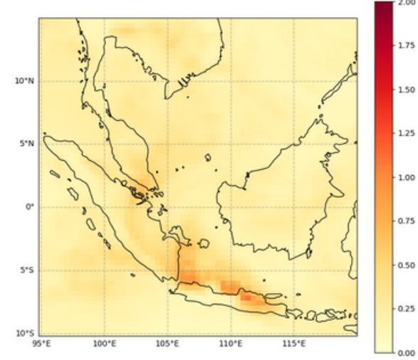
Total Aerosol Optical Depth at 550 nm, 2023-06-25T00
