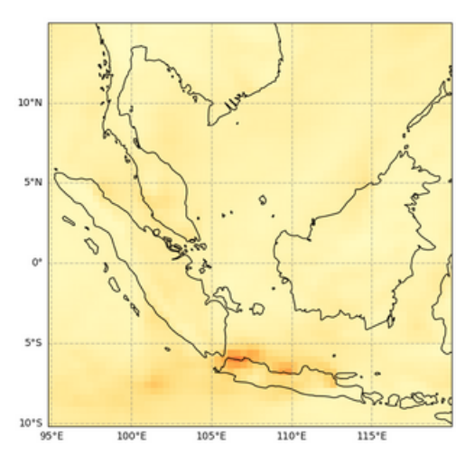
Total Aerosol Optical Depth at 550 nm, 2023-06-15T00
