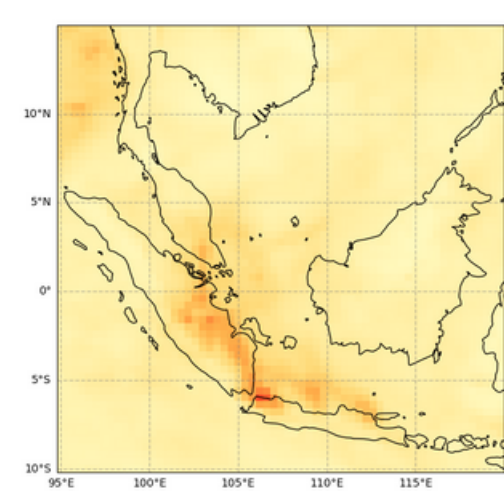
Total Aerosol Optical Depth at 550 nm, 2023-06-06T00
