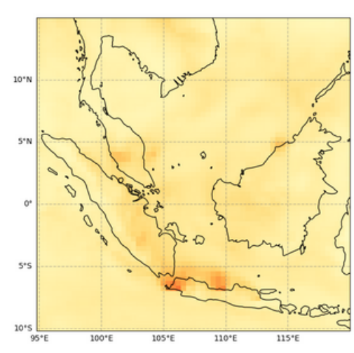
Total Aerosol Optical Depth at 550 nm, 2023-06-03T00
