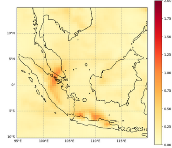
Total Aerosol Optical Depth at 550 nm, 2023-06-24T00
