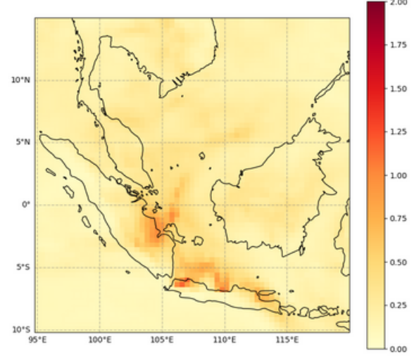
Total Aerosol Optical Depth at 550 nm, 2023-06-26T00
