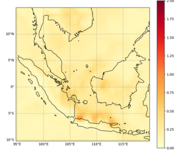
Total Aerosol Optical Depth at 550 nm, 2023-06-27T00
