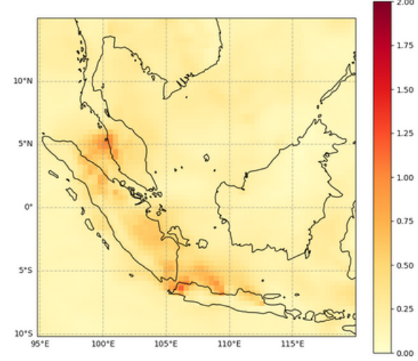
Total Aerosol Optical Depth at 550 nm, 2023-06-22T00
