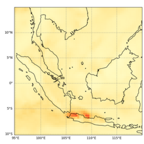
Total Aerosol Optical Depth at 550 nm, 2023-06-14T00
