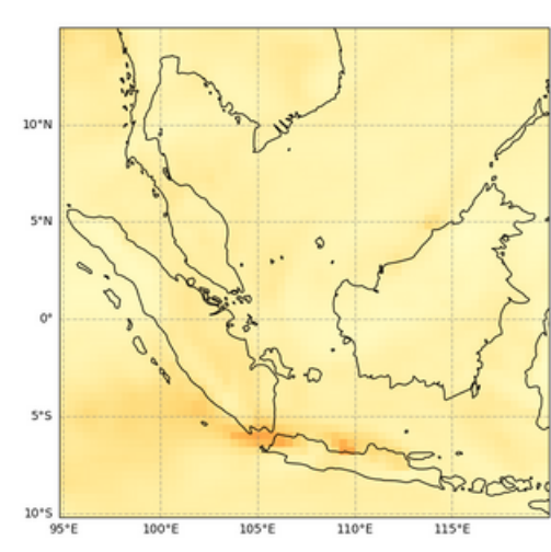
Total Aerosol Optical Depth at 550 nm, 2023-06-13T00
