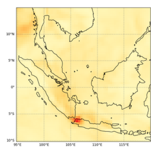
Total Aerosol Optical Depth at 550 nm, 2023-06-07T00
