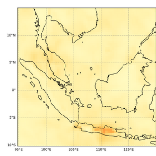
Total Aerosol Optical Depth at 550 nm, 2023-06-17T00
