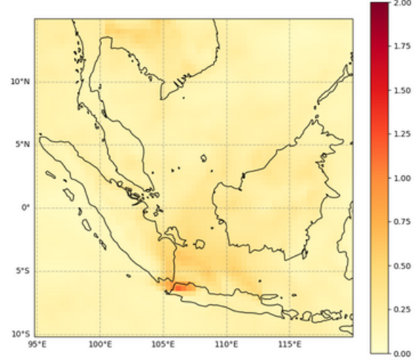
Total Aerosol Optical Depth at 550 nm, 2023-06-28T00
