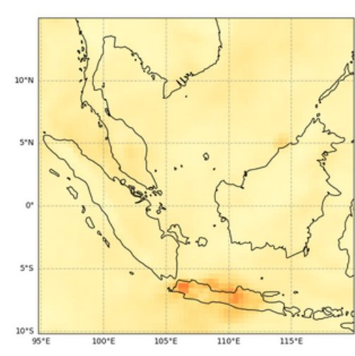
Total Aerosol Optical Depth at 550 nm, 2023-06-16T00
