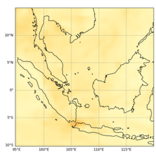
Total Aerosol Optical Depth at 550 nm, 2023-06-08T00
