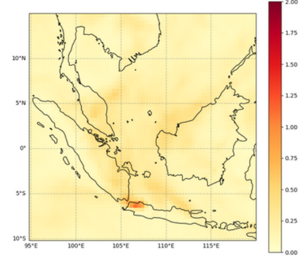
Total Aerosol Optical Depth at 550 nm, 2023-06-30T00
