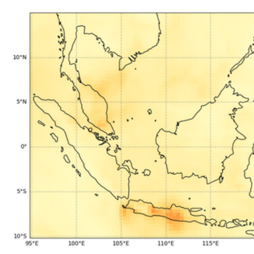
Total Aerosol Optical Depth at 550 nm, 2023-06-18T00
