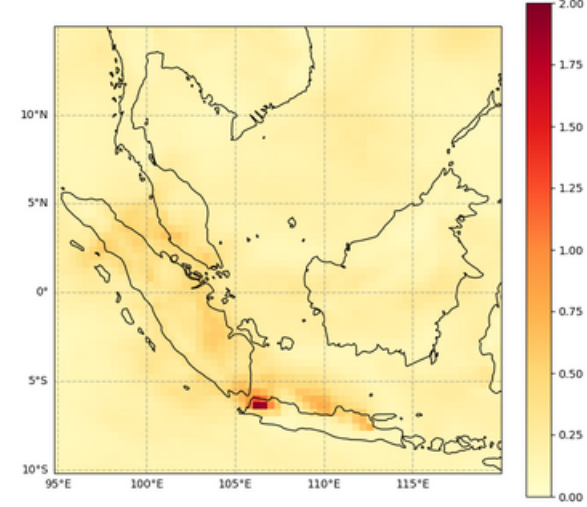
Total Aerosol Optical Depth at 550 nm, 2023-06-23T00
