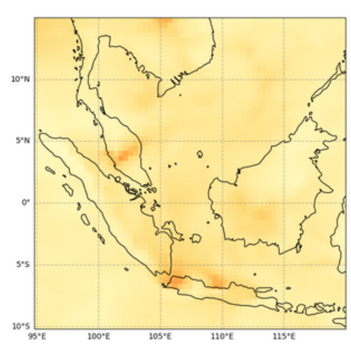
Total Aerosol Optical Depth at 550 nm, 2023-06-02T00
