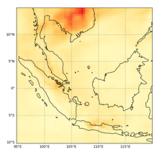
Total Aerosol Optical Depth at 550 nm, 2023-04-01T00
