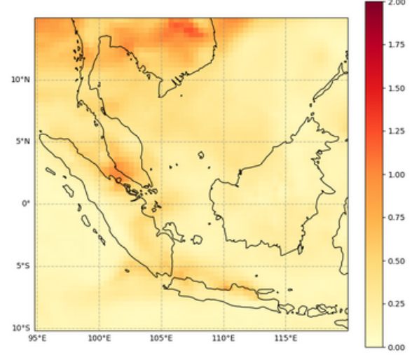
Total Aerosol Optical Depth at 550 nm, 2023-04-20T00
