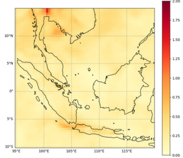
Total Aerosol Optical Depth at 550 nm, 2023-04-28T00
