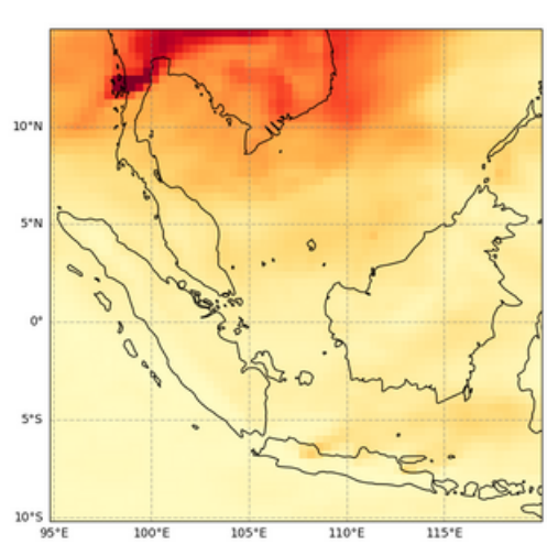
Total Aerosol Optical Depth at 550 nm, 2023-04-10T00
