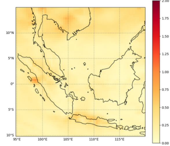
Total Aerosol Optical Depth at 550 nm, 2023-04-25T00
