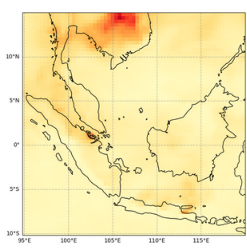
Total Aerosol Optical Depth at 550 nm, 2023-04-02T00
