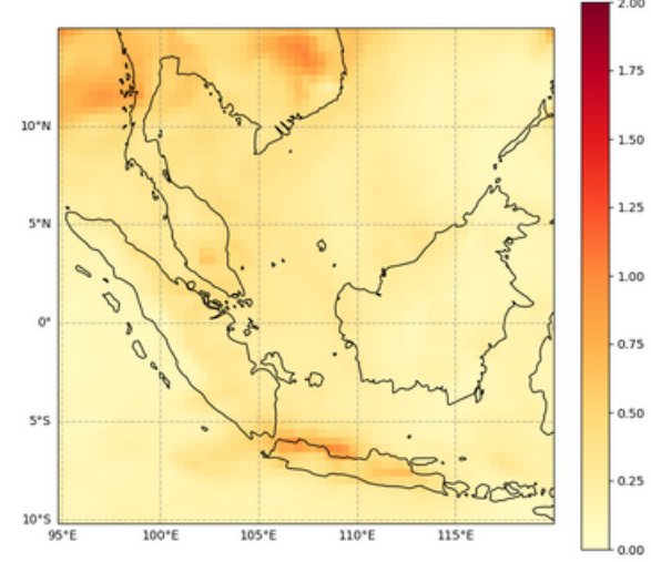
Total Aerosol Optical Depth at 550 nm, 2023-04-22T00
