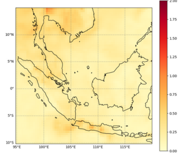
Total Aerosol Optical Depth at 550 nm, 2023-04-29T00
