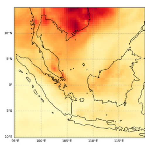
Total Aerosol Optical Depth at 550 nm, 2023-04-15T00
