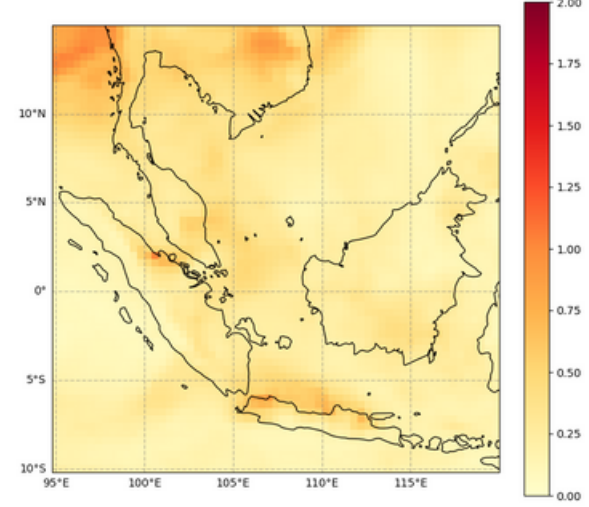
Total Aerosol Optical Depth at 550 nm, 2023-04-21T00
