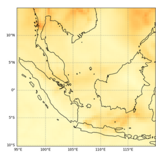
Total Aerosol Optical Depth at 550 nm, 2023-04-07T00
