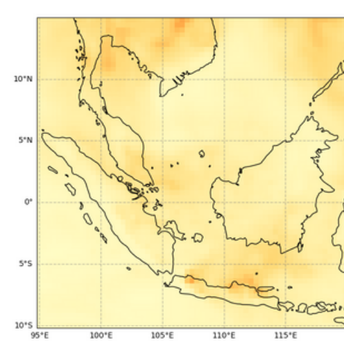
Total Aerosol Optical Depth at 550 nm, 2023-04-06T00
