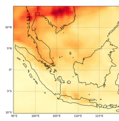
Total Aerosol Optical Depth at 550 nm, 2023-04-18T00
