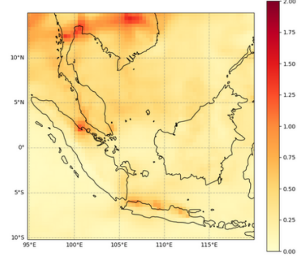
Total Aerosol Optical Depth at 550 nm, 2023-04-19T00
