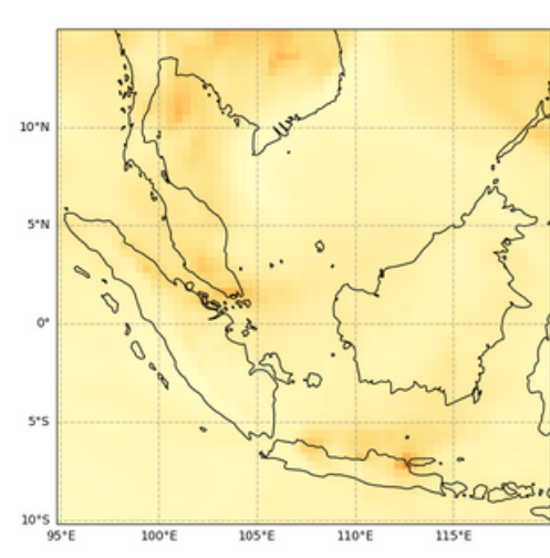
Total Aerosol Optical Depth at 550 nm, 2023-04-05T00
