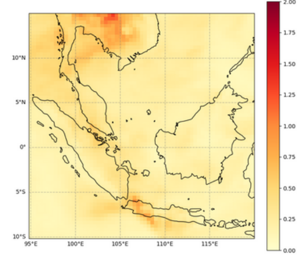
Total Aerosol Optical Depth at 550 nm, 2023-04-30T00
