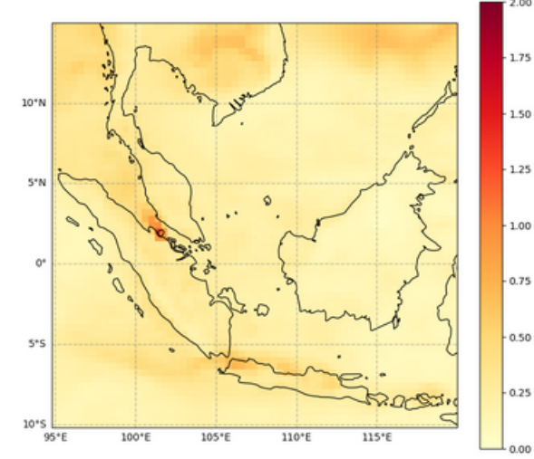
Total Aerosol Optical Depth at 550 nm, 2023-04-24T00
