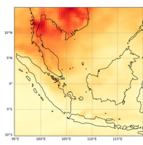
Total Aerosol Optical Depth at 550 nm, 2023-04-12T00
