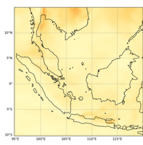
Total Aerosol Optical Depth at 550 nm, 2023-04-04T00
