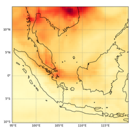
Total Aerosol Optical Depth at 550 nm, 2023-04-14T00
