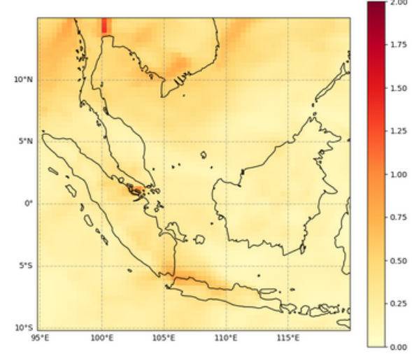
Total Aerosol Optical Depth at 550 nm, 2023-04-27T00
