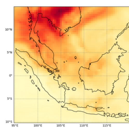
Total Aerosol Optical Depth at 550 nm, 2023-04-17T00
