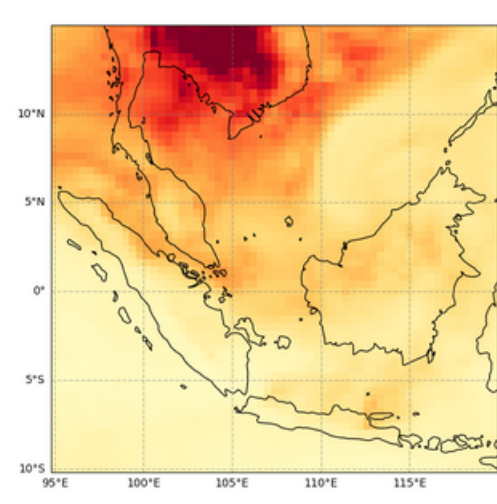
Total Aerosol Optical Depth at 550 nm, 2023-04-16T00
