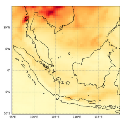
Total Aerosol Optical Depth at 550 nm, 2023-04-09T00
