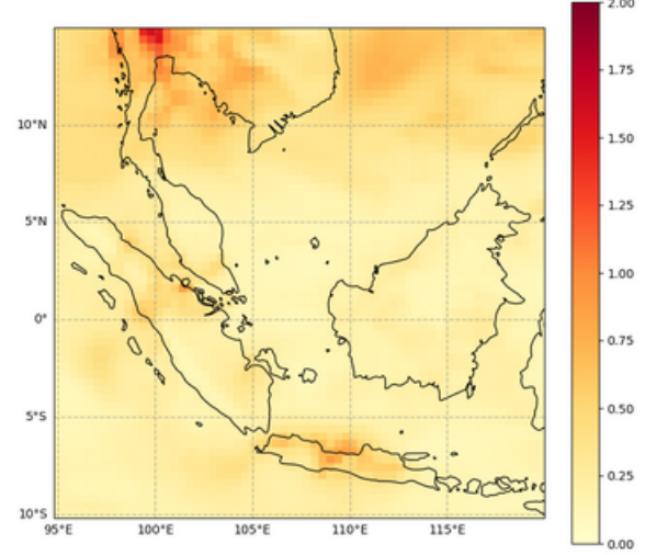
Total Aerosol Optical Depth at 550 nm, 2023-04-26T00
