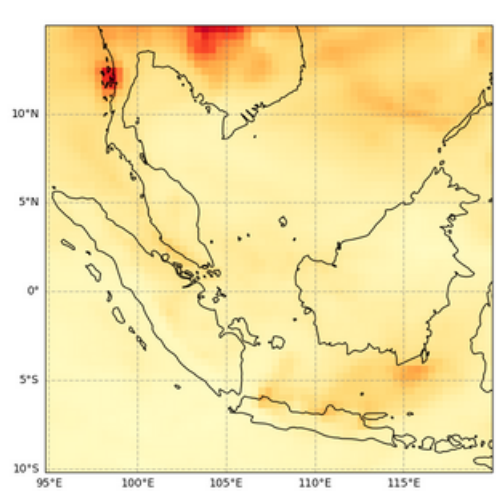
Total Aerosol Optical Depth at 550 nm, 2023-04-08T00
