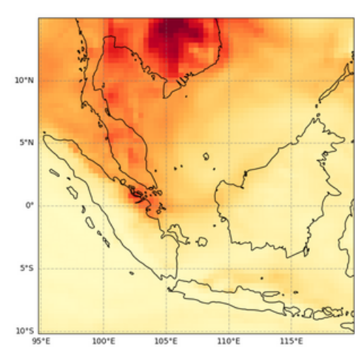
Total Aerosol Optical Depth at 550 nm, 2023-04-13T00
