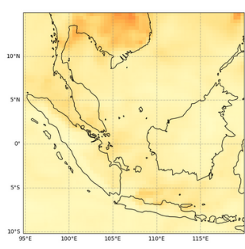
Total Aerosol Optical Depth at 550 nm, 2023-04-03T00
