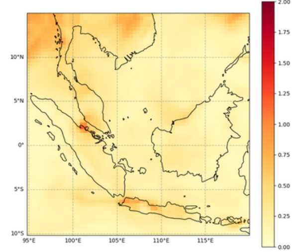
Total Aerosol Optical Depth at 550 nm, 2023-04-23T00
