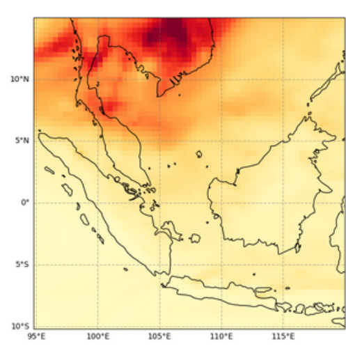
Total Aerosol Optical Depth at 550 nm, 2023-04-11T00
