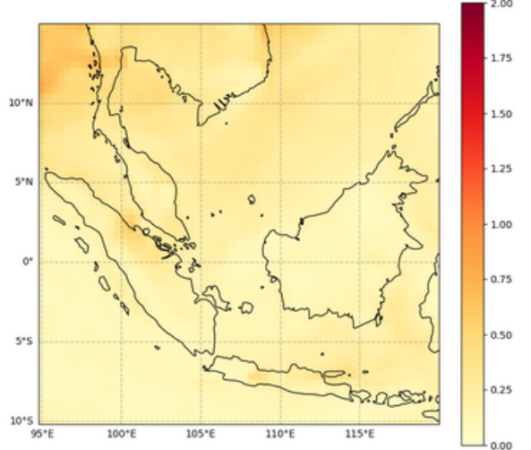
Total Aerosol Optical Depth at 550 nm, 2023-03-05T00
