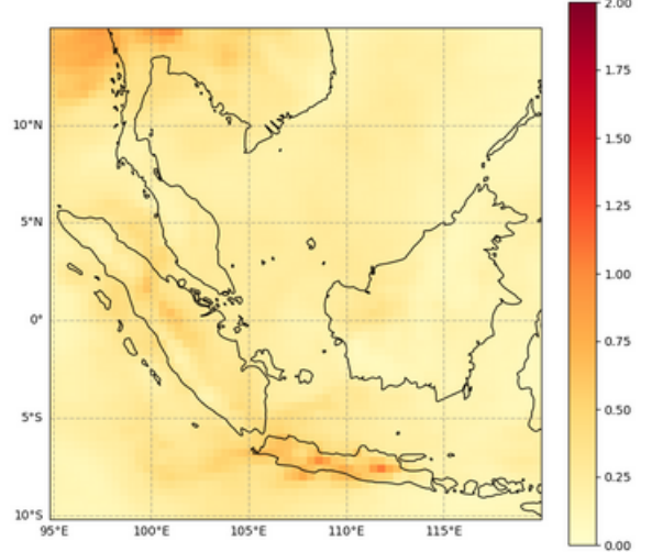
Total Aerosol Optical Depth at 550 nm, 2023-03-17T00
