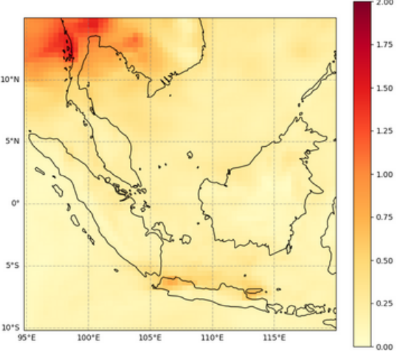
Total Aerosol Optical Depth at 550 nm, 2023-03-12T00
