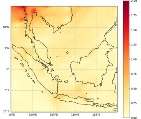
Total Aerosol Optical Depth at 550 nm, 2023-03-10T00
