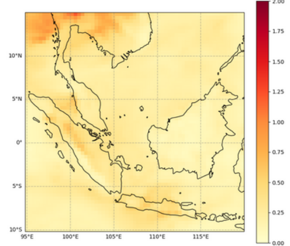
Total Aerosol Optical Depth at 550 nm, 2023-03-16T00
