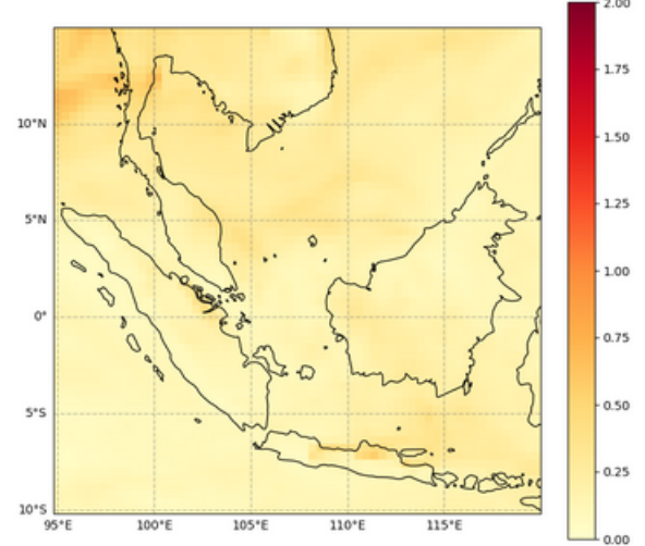
Total Aerosol Optical Depth at 550 nm, 2023-03-04T00
