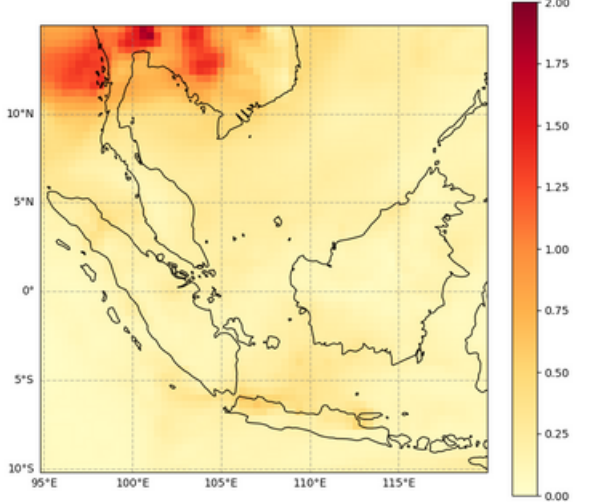
Total Aerosol Optical Depth at 550 nm, 2023-03-11T00
