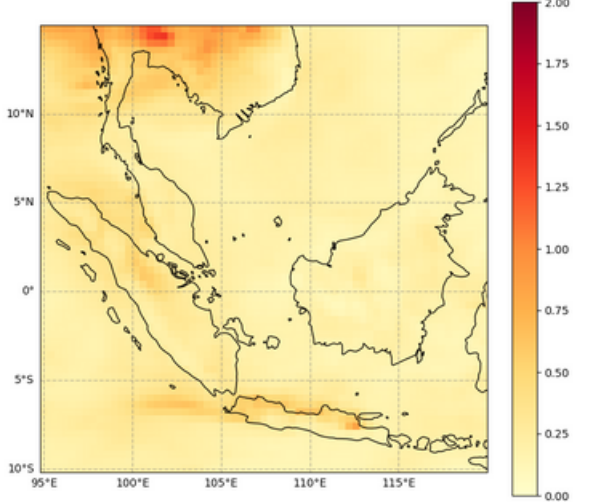
Total Aerosol Optical Depth at 550 nm, 2023-03-18T00
