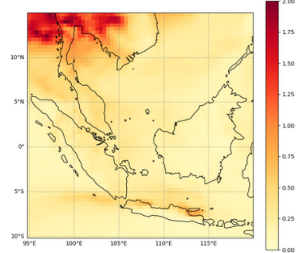
Total Aerosol Optical Depth at 550 nm, 2023-03-13T00
