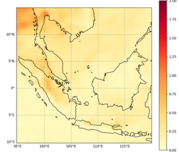
Total Aerosol Optical Depth at 550 nm, 2023-03-07T00
