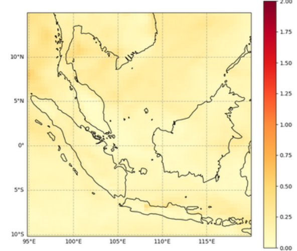
Total Aerosol Optical Depth at 550 nm, 2023-03-01T00
