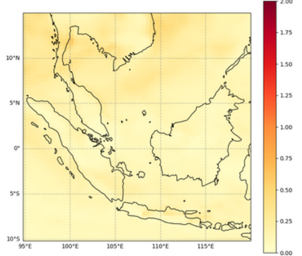
Total Aerosol Optical Depth at 550 nm, 2023-03-02T00
