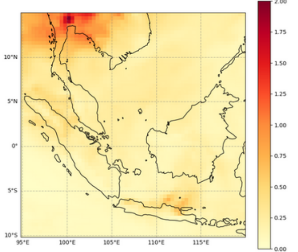
Total Aerosol Optical Depth at 550 nm, 2023-03-09T00
