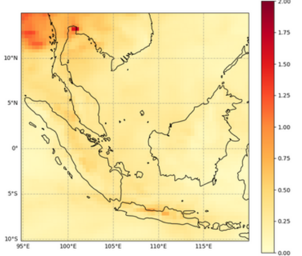
Total Aerosol Optical Depth at 550 nm, 2023-03-15T00
